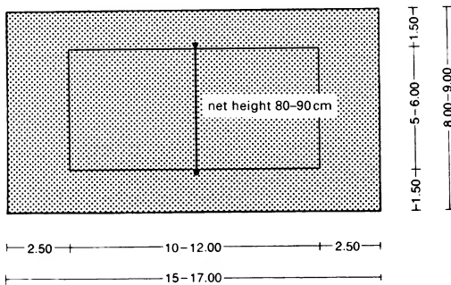
③ Children's tennis court
